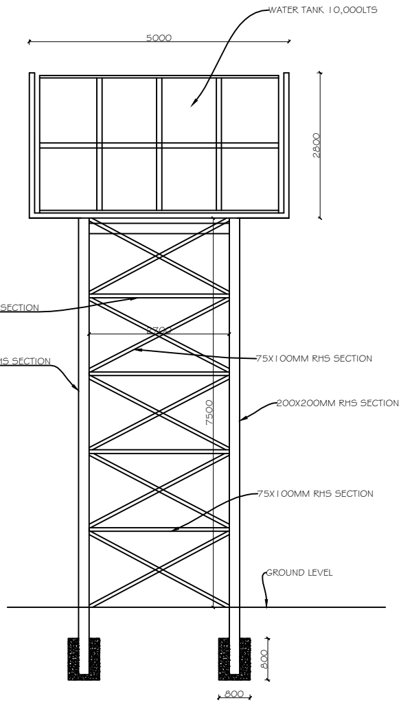
SECTION
