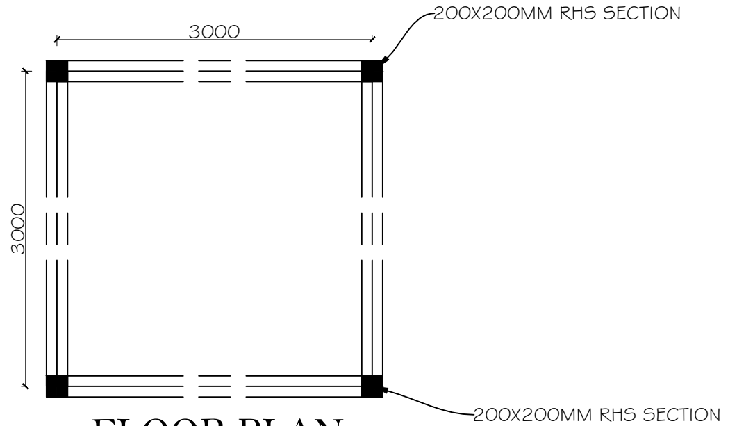
FLOOR PLAN
